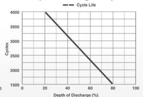
Depth of Discharge vs. Cycles
